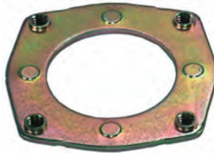
230907 Bearing Plate Replacing: 021411-0480 Servicing: 100210-3070, 100210-3190, 100210-3210, 100210-3380, 100210-3381, 100210-3410, 100210-3470, 100210-3480, 100210-3700 ID 30.00, OD 48.00x48.00, Thickness 2.85, Dist. mount. holes 42.00, No./mount. holes 4, Gasket w/o
