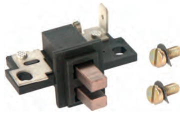
130933 Brush Box Replacing: ULB653, ULB650 14 Volt, OD 44.80
