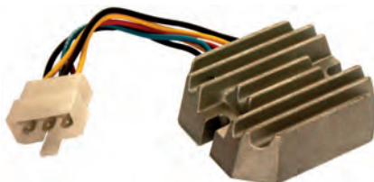
234414 Regulator/Rectifier Replacing: AM126304 14 Volt, Dist. mount. holes 62.50, Regulator type Electronic Terminals: B+(red), IG(red/blue), -(black), AC(yellow), L(brown), AC(yellow).
