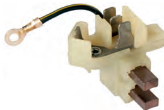
131703 Brush Box Replacing: ULB812 Servicing: A125 14 Volt, OD 47.90
