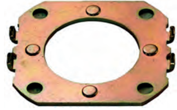
230996# Bearing Plate Replacing: 021411-0500 Servicing: 100211-1440, 100211-1511, 100211-1512, 100211-1520, 100211-1540, 100211-1550, 100211-1560, 100211-1570, 100211-1571 ID 28.00, OD 43.60x44.90, Thickness 2.00, Dist. mount. holes 33.30, No./mount. holes 4, Gasket w/o
