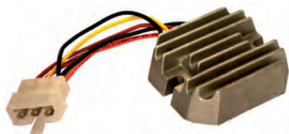
234412 Regulator/Rectifier Replacing: RS5160 14 Volt, 20 Amp, Dist. mount. holes 63.55 20 A charging system. Terminals: B+(red), IG(yellow), B-(black), AC(orange), L(brown), AC(orange).
