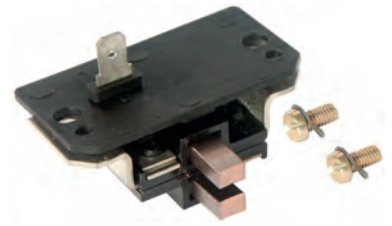
131704 Brush Box Replacing: ULB237 14 Volt, OD 54.00
