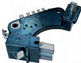
135446# Brush Box
